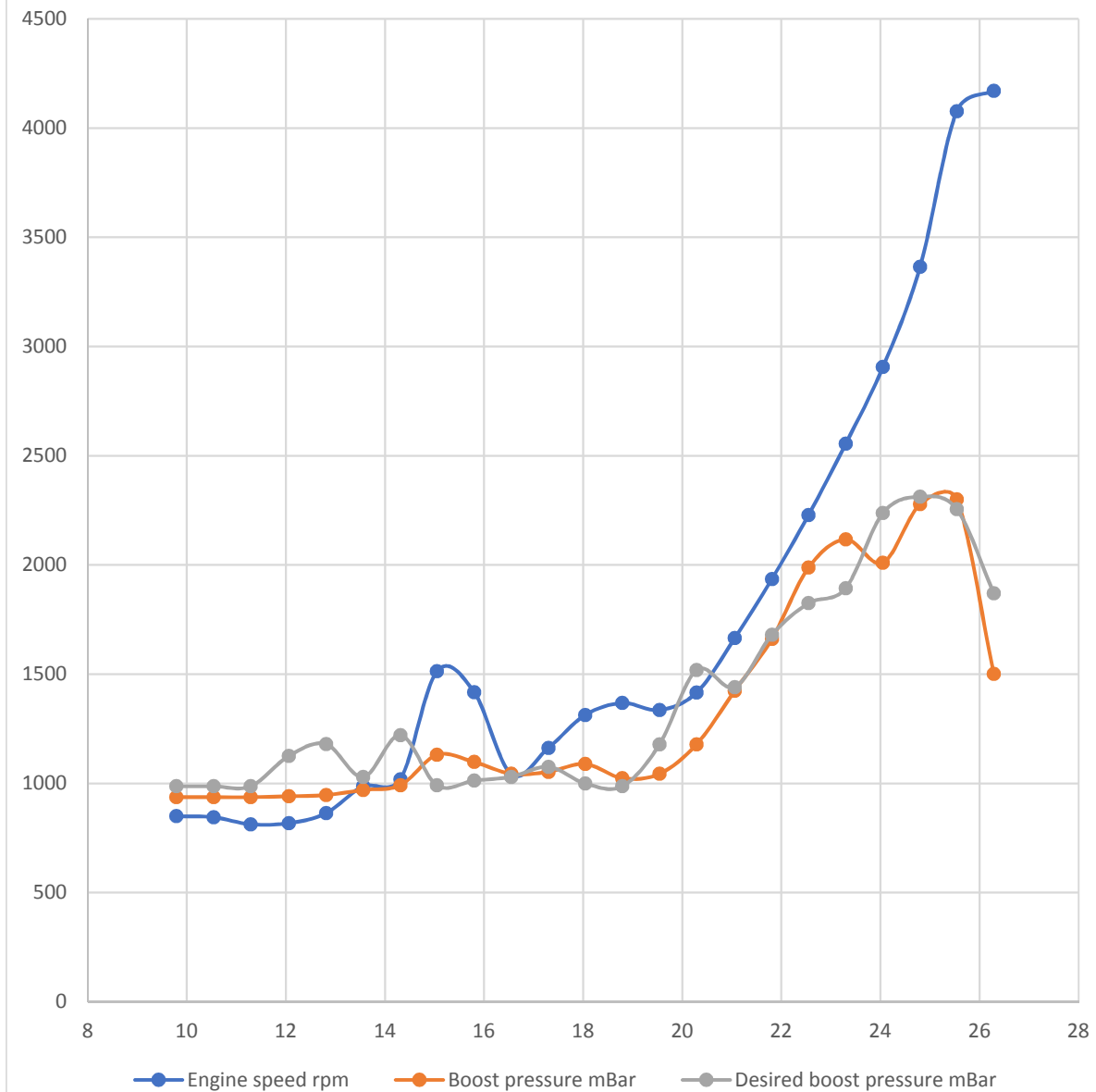
Boost pressure
